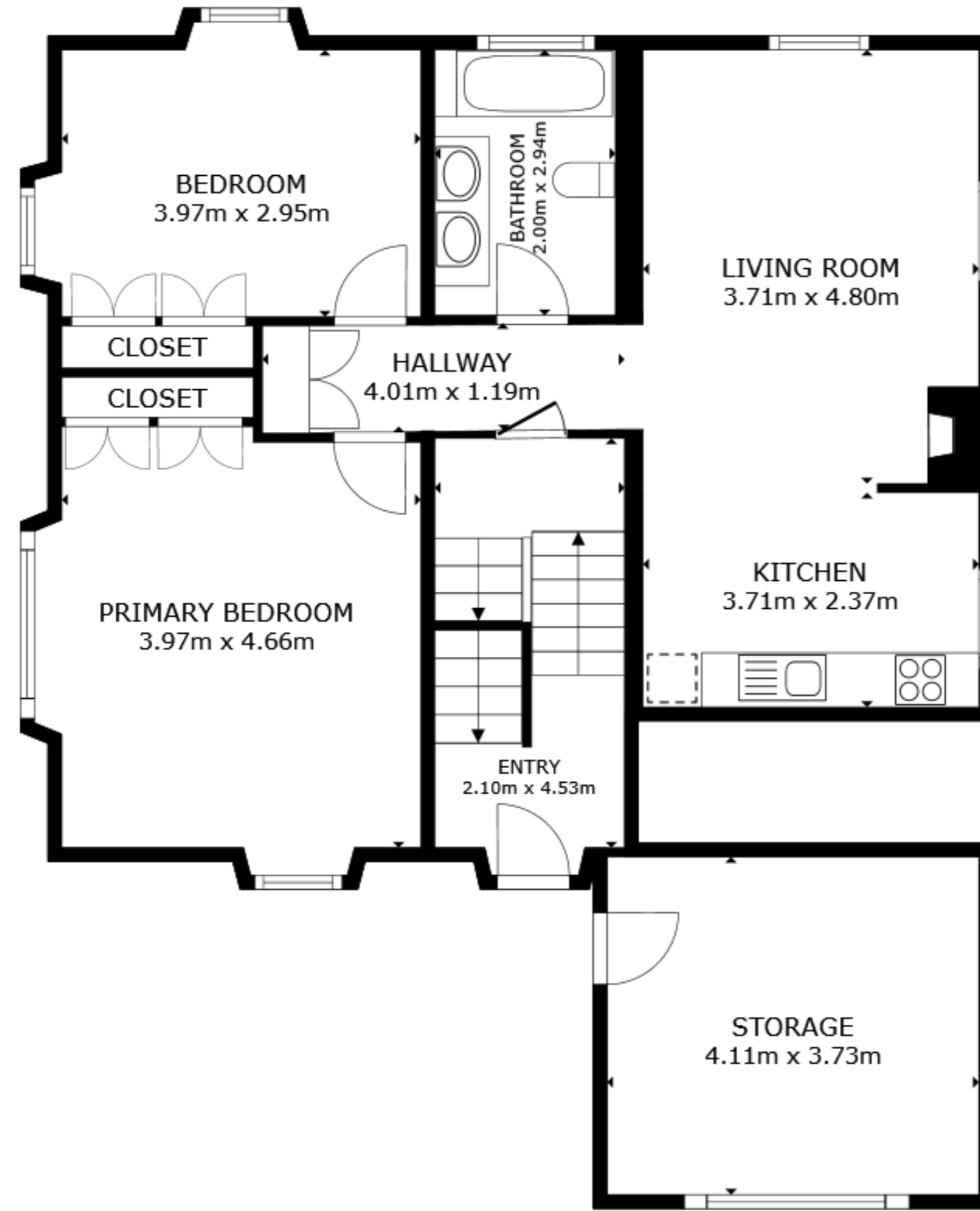
FLOOR 2
