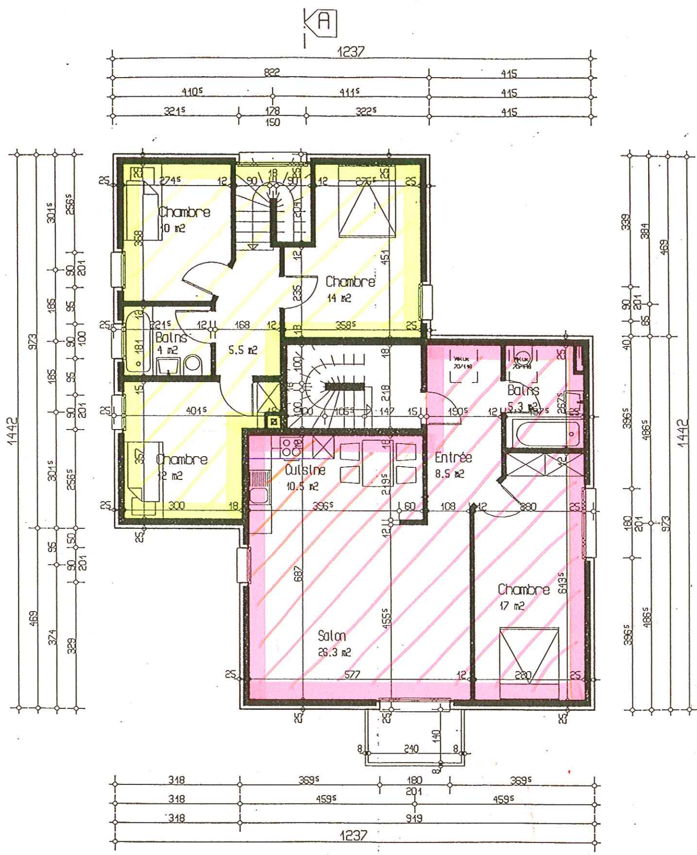
A ETAGE VILLA type "D" Duplex 4.5 pos 2.5 pos et. 1.
