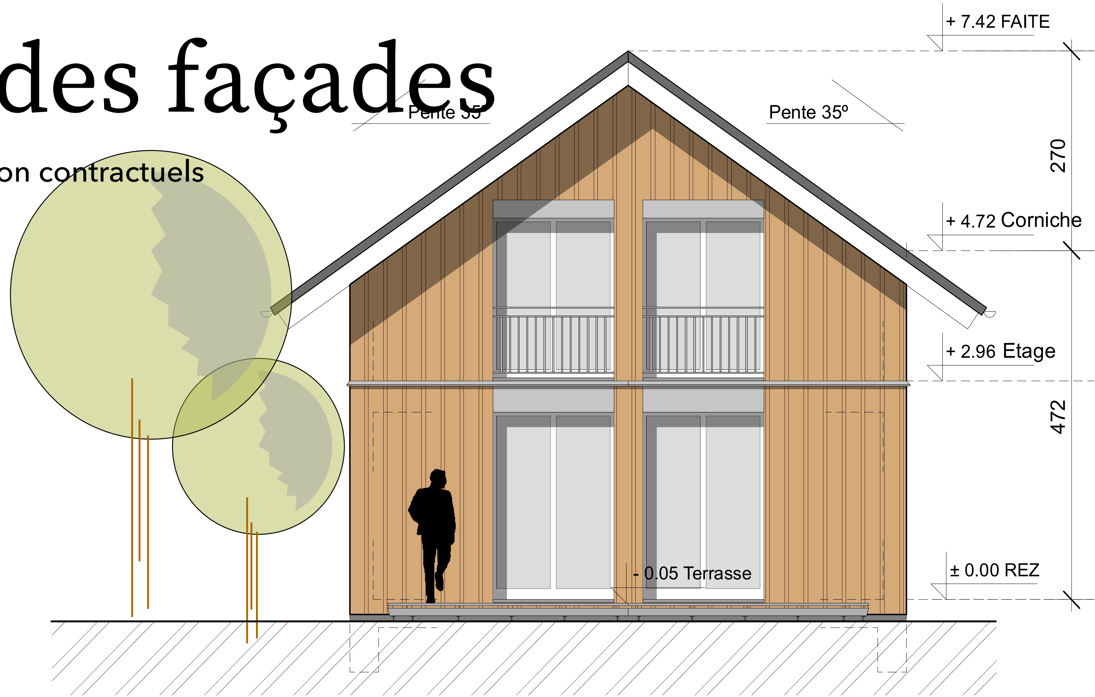
FACADE SUD
