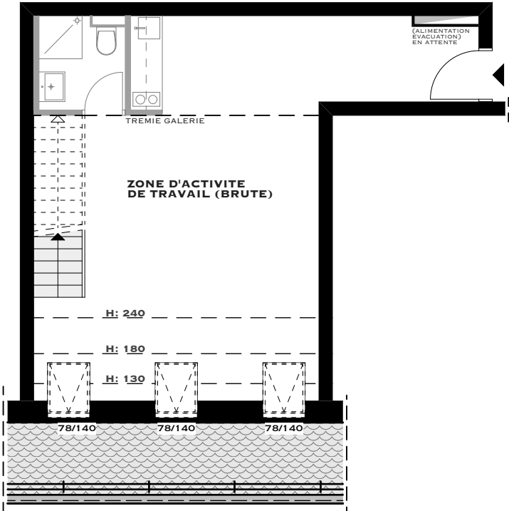
PLAN COMBLES ECH _ 1/100
