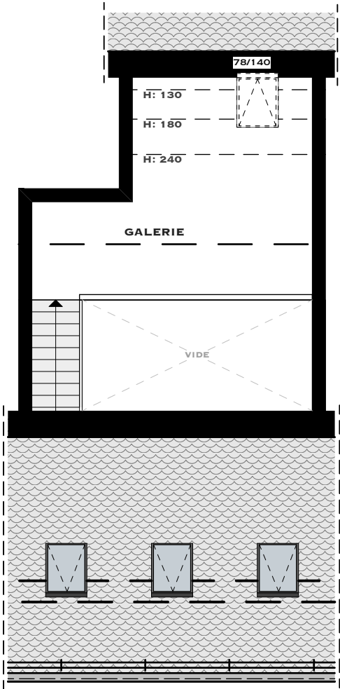
PLAN SURCOMBLES ECH _ 1/100
