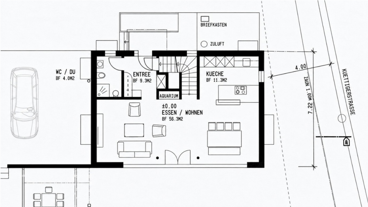
ATTIKAGESCHOSS
