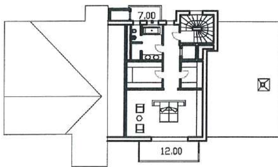
PLAN COMBLES 90.00
