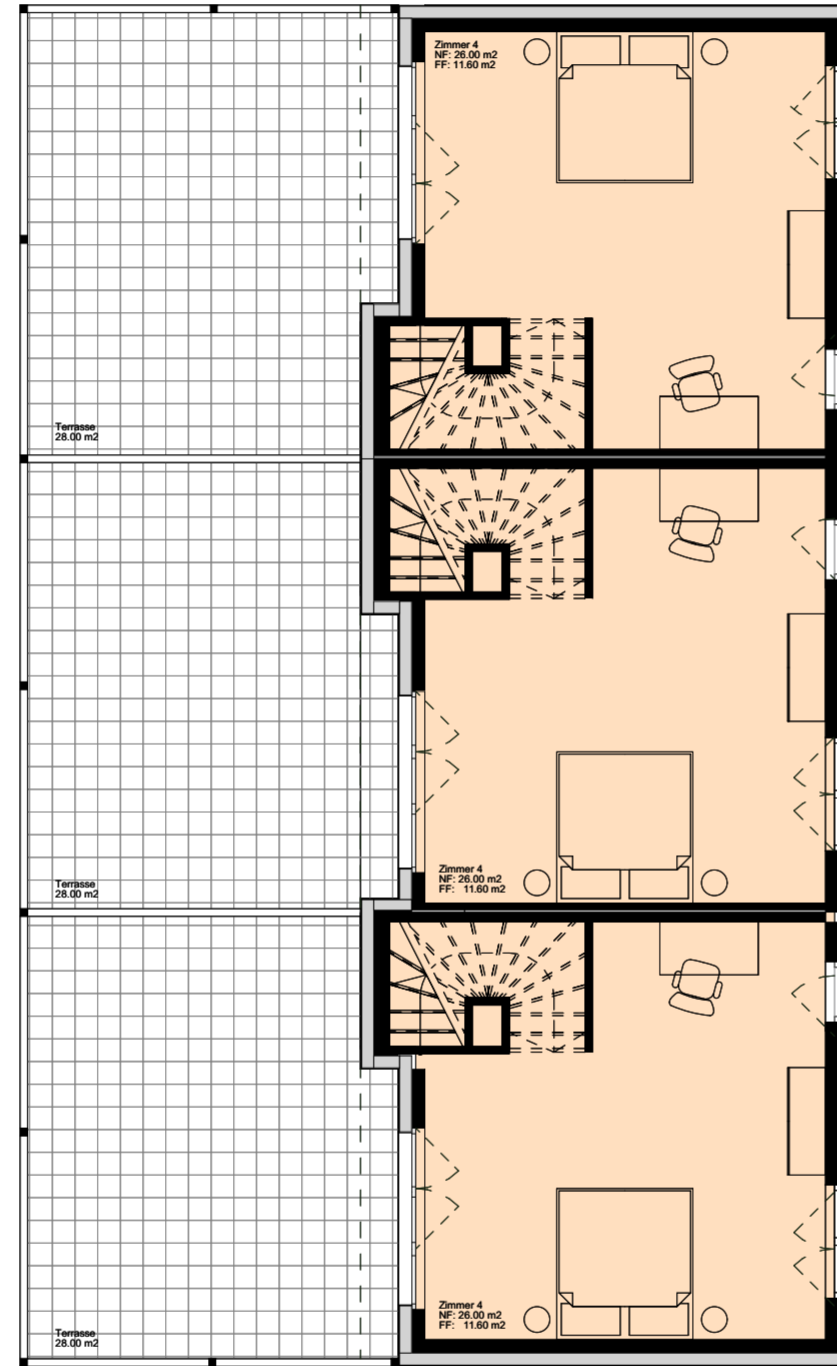
Grundriss Attikageschoss
