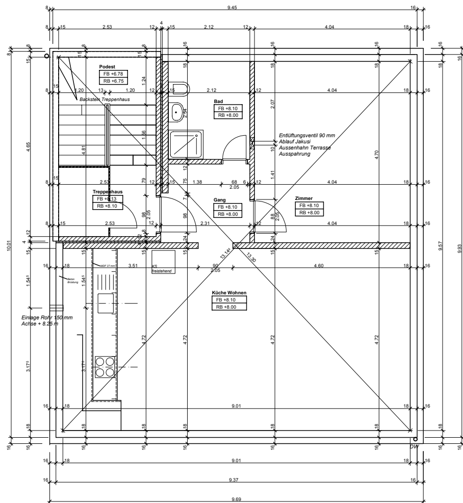
Grundriss DG 1: 100
