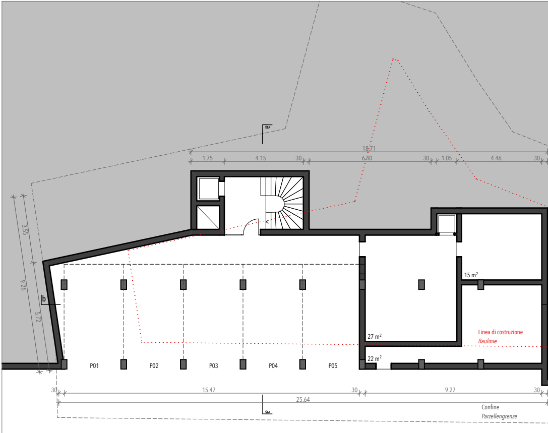
Pian terreno | Erdgeschoss
