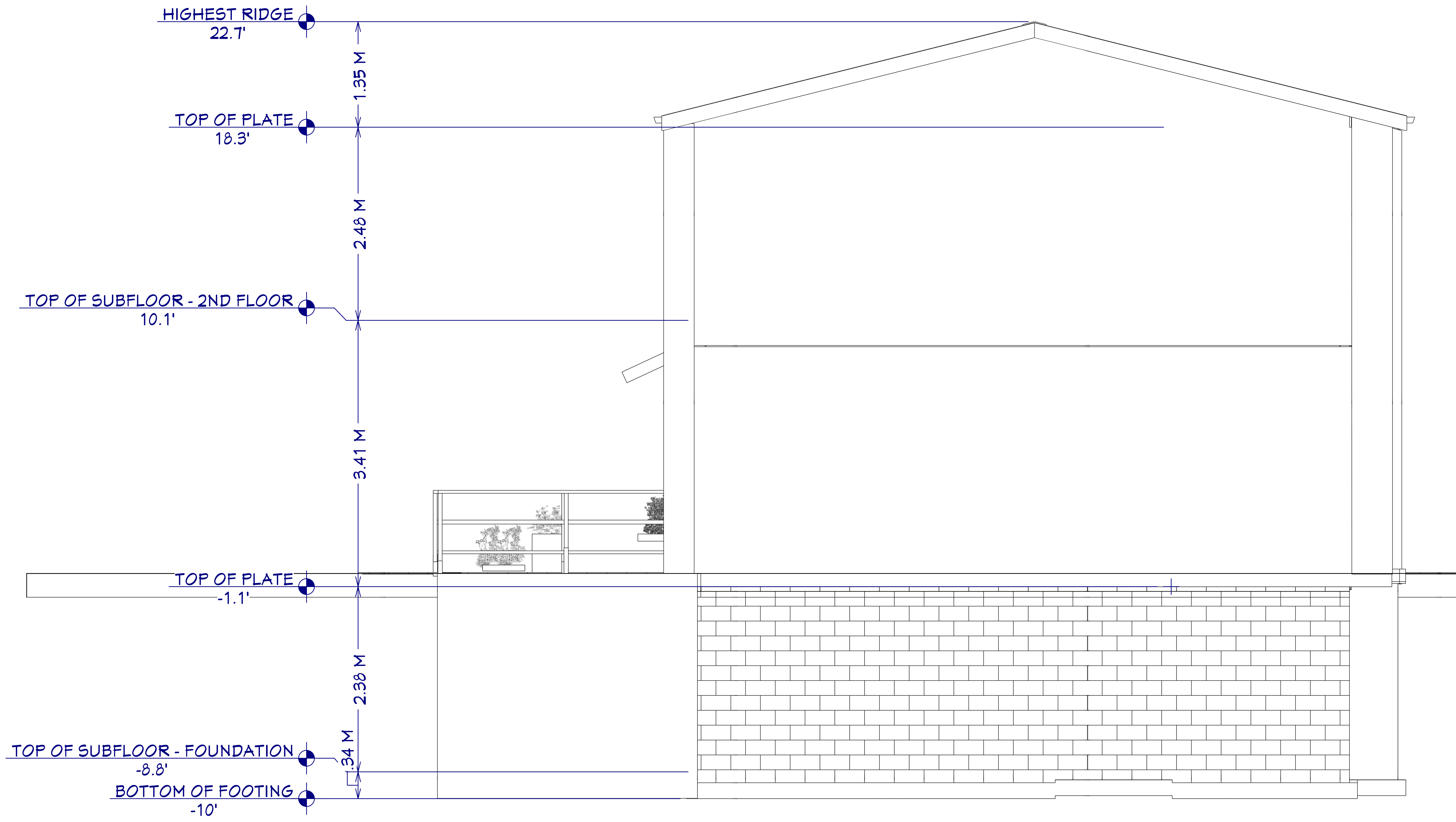
E2 ELEVATION 2 1/2 IN = 1 FT
