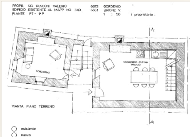
ERDGESCHOSS · PIANTA PIANO TERRENO — MST. 1:50
