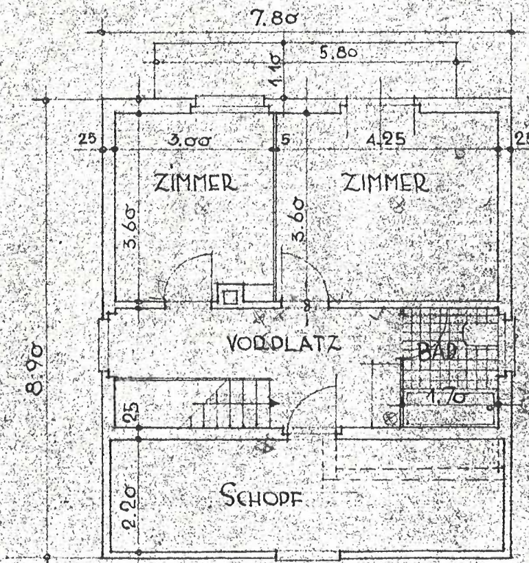
1. STOCK
