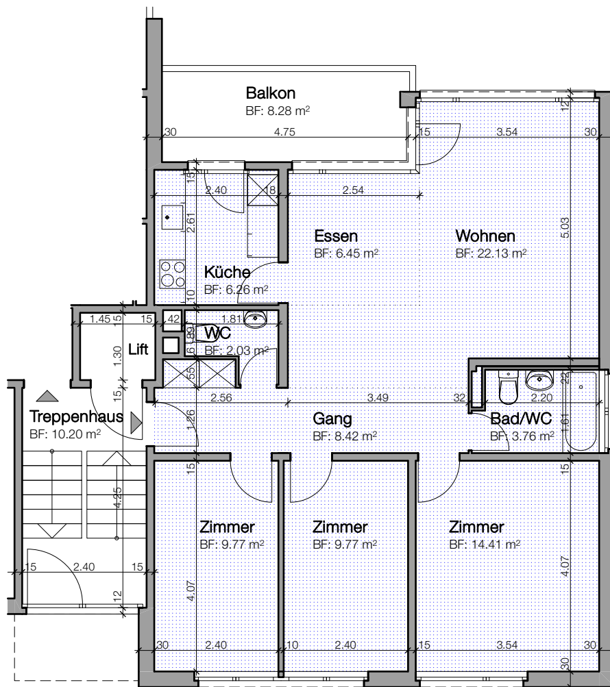
NWF 4½-Zi-Whg BF: 83.00 m²
