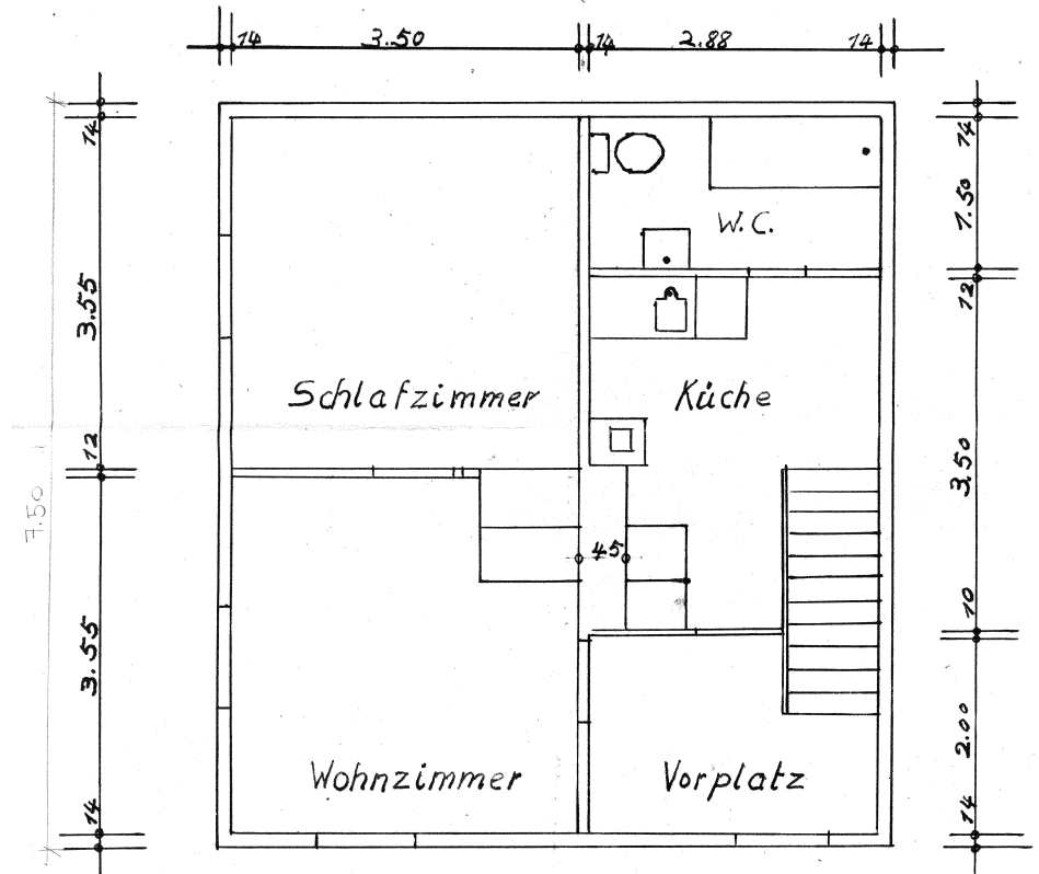
Grundriss Partere
