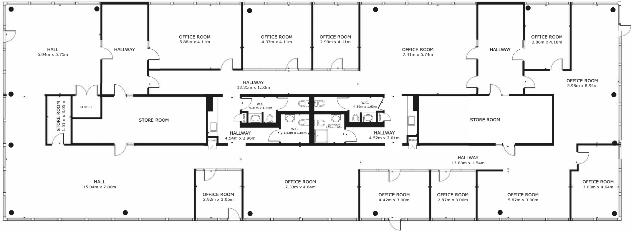
FLOOR PLAN
