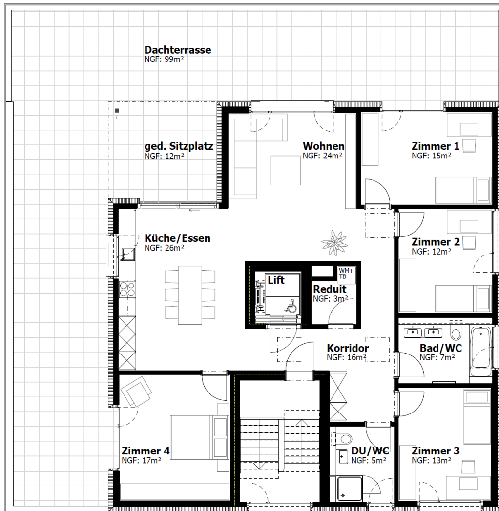
Grundriss Attikageschoss
