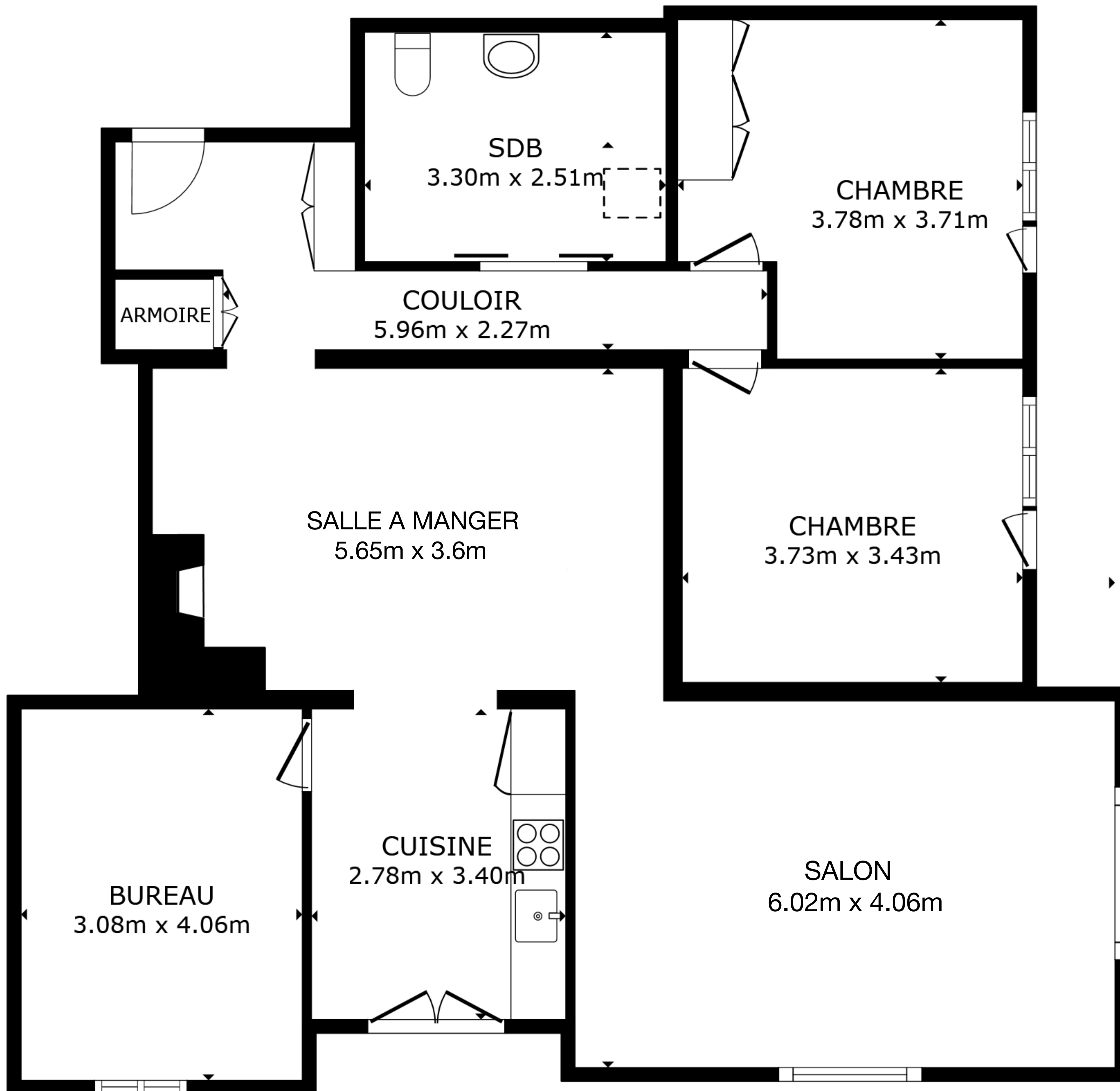
FLOOR PLAN
