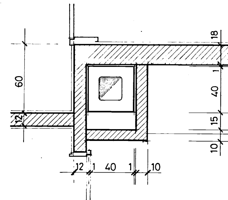
detail A 1:20
