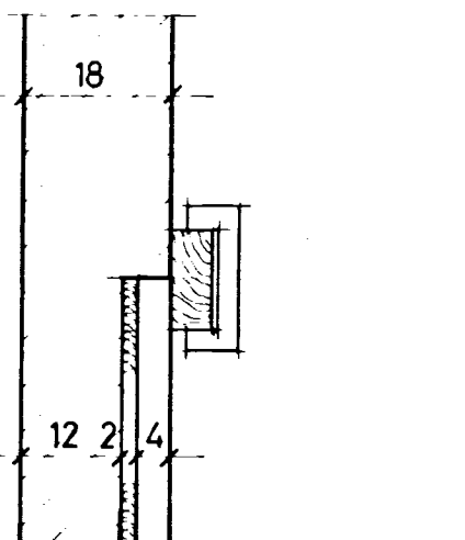
detail D Mst.1:10
