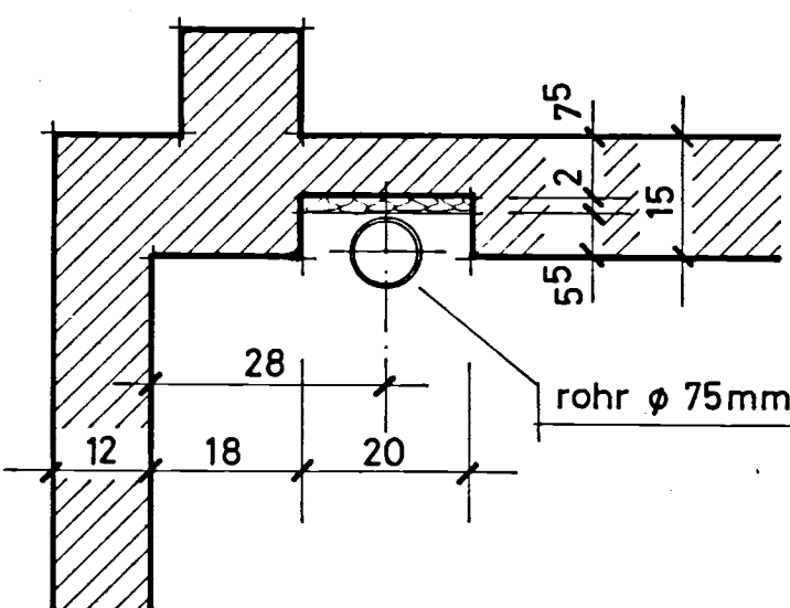
detail Ms 1:10
