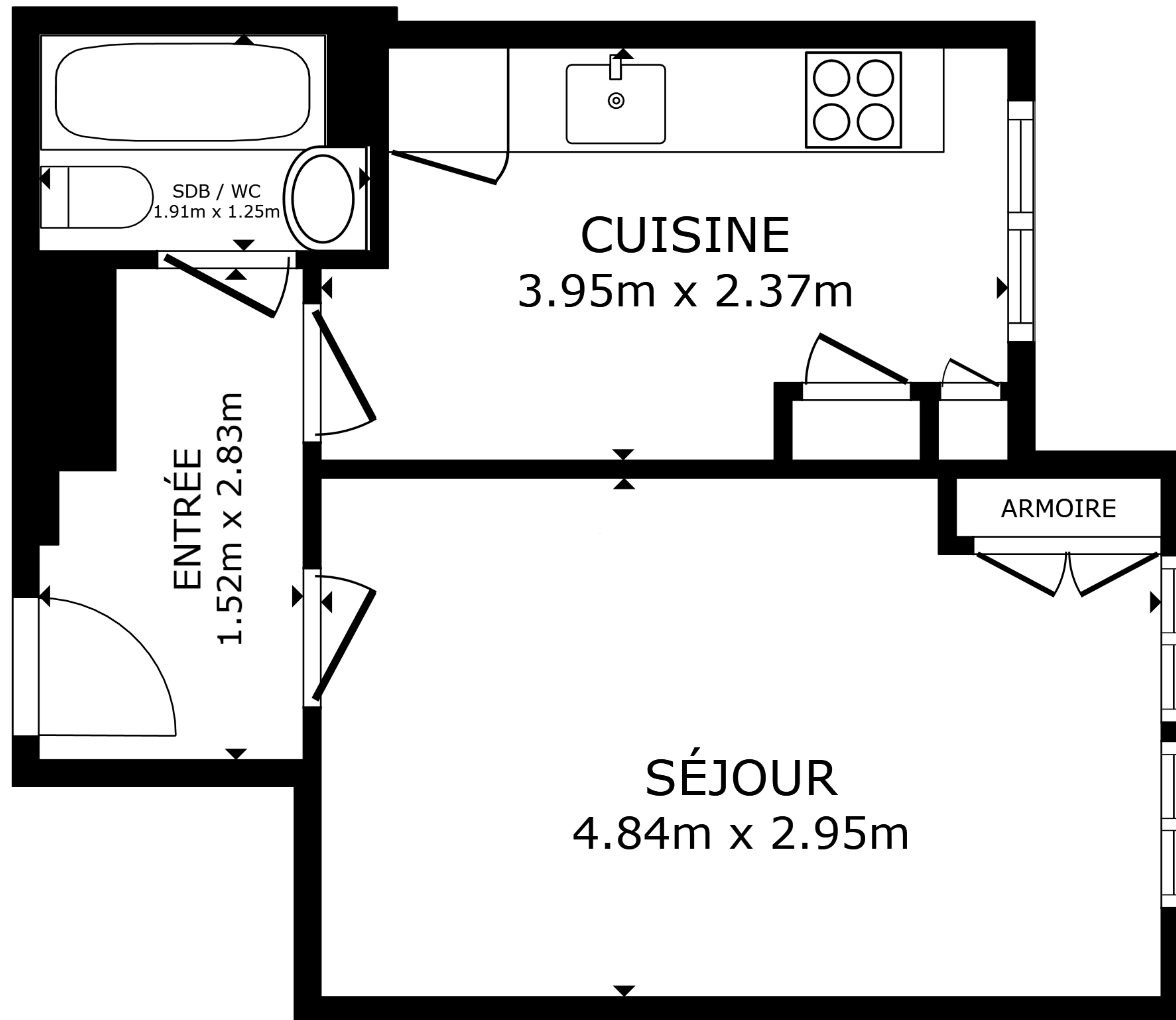
FLOOR PLAN
