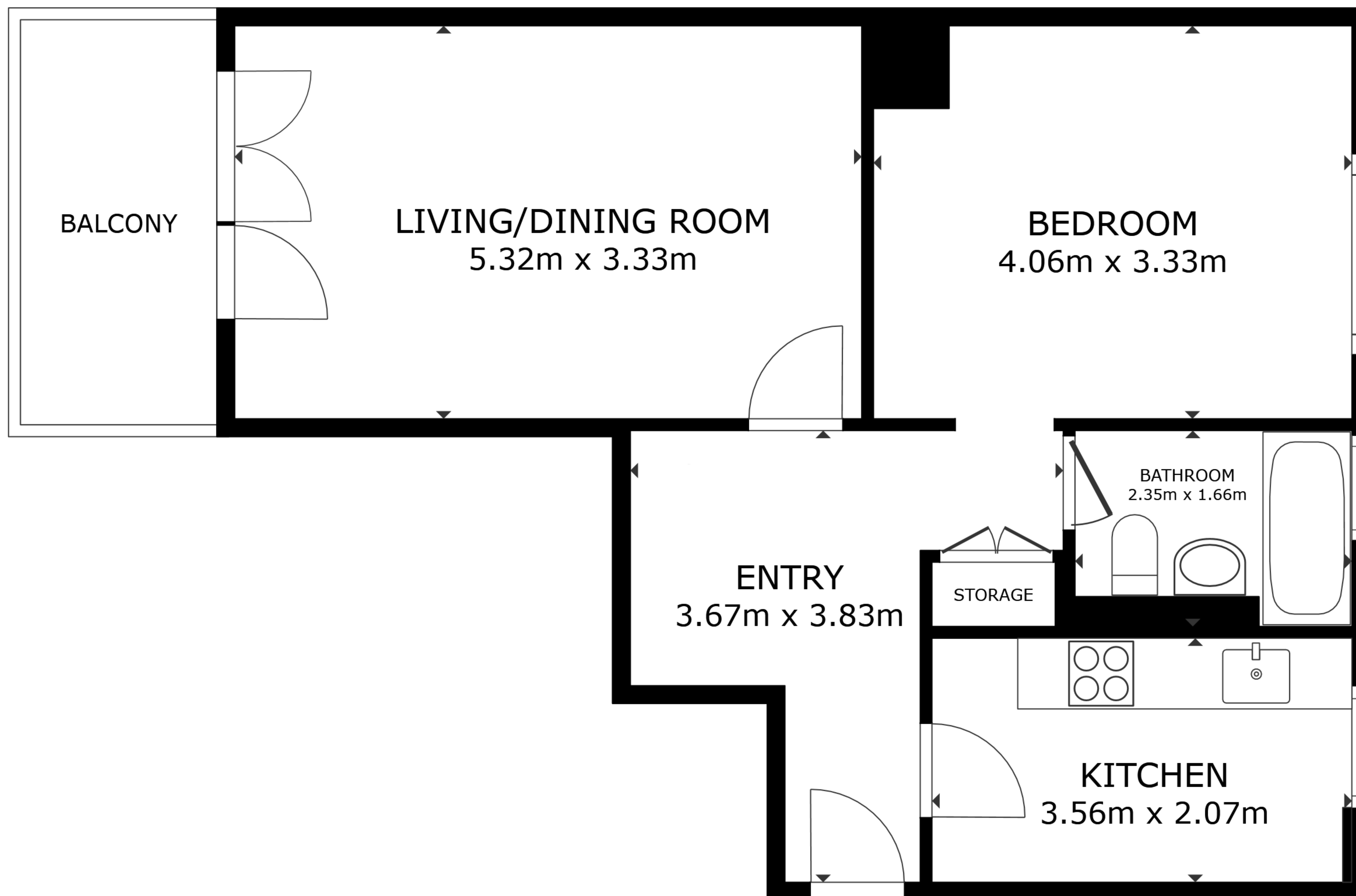
FLOOR PLAN
