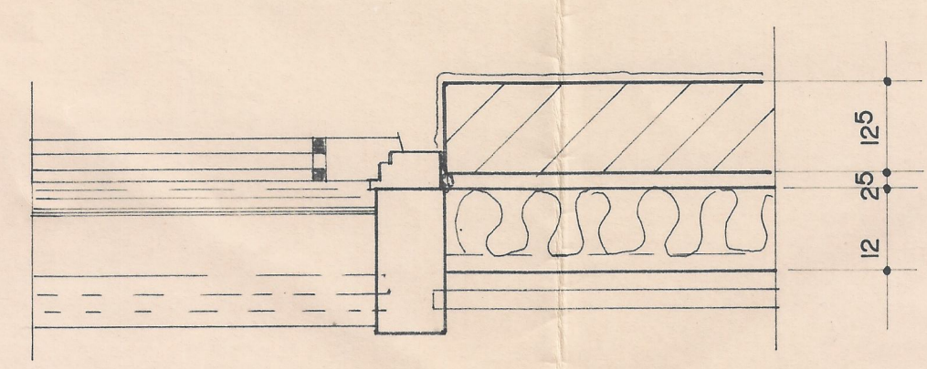
DETAIL III 1:10
