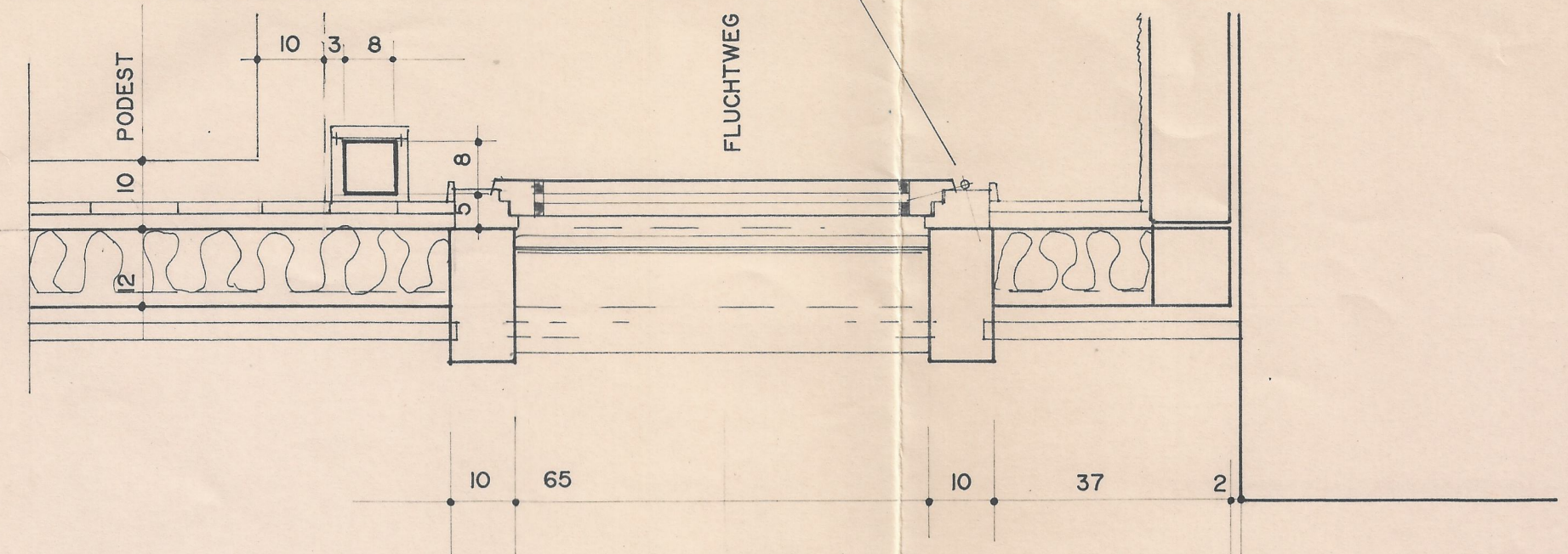
DETAIL IV 1:10
