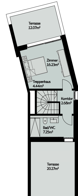
Attikageschoss
