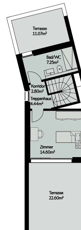
Attikageschoss
