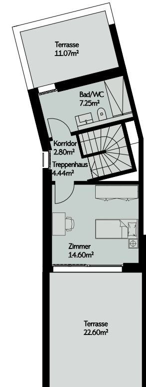
Attikageschoss
