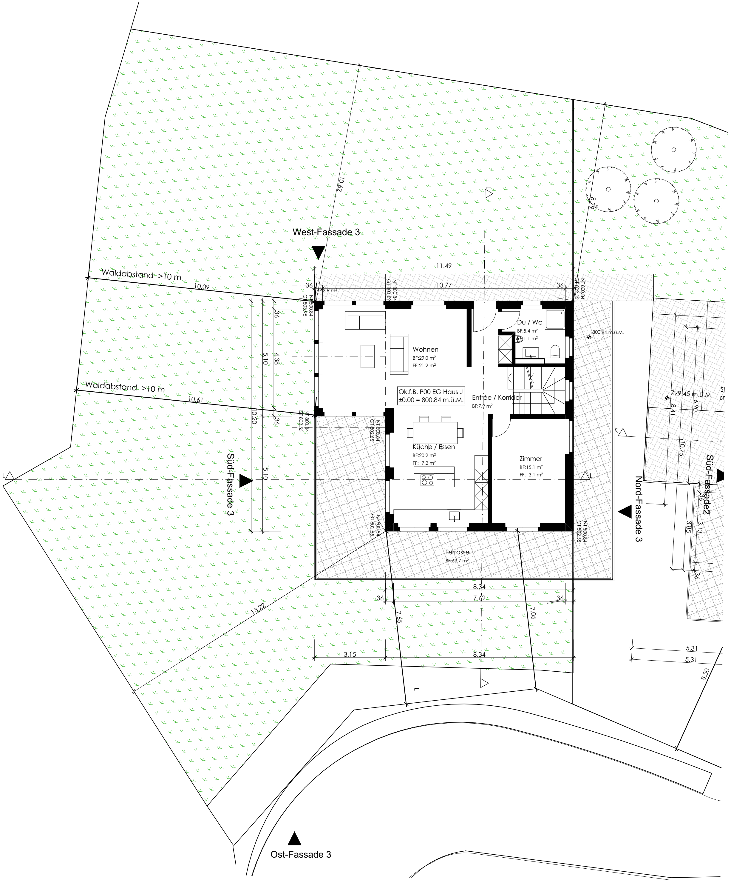
P00 Erdgeschoss
