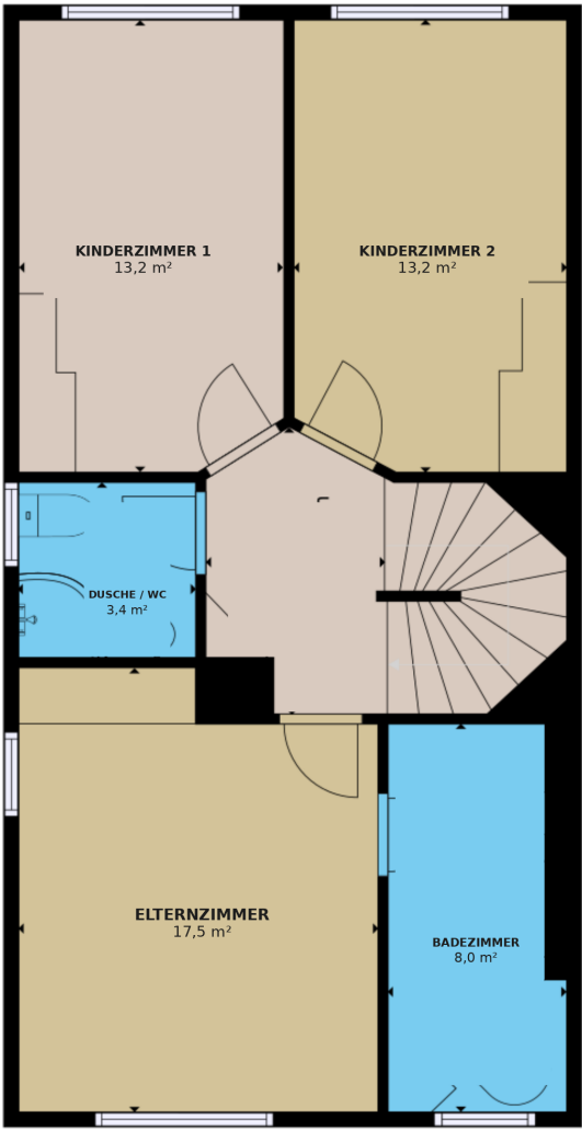
OBERGESCHOSS (OG)
